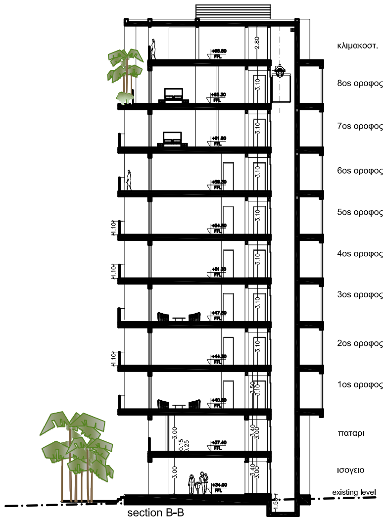
section B-B
