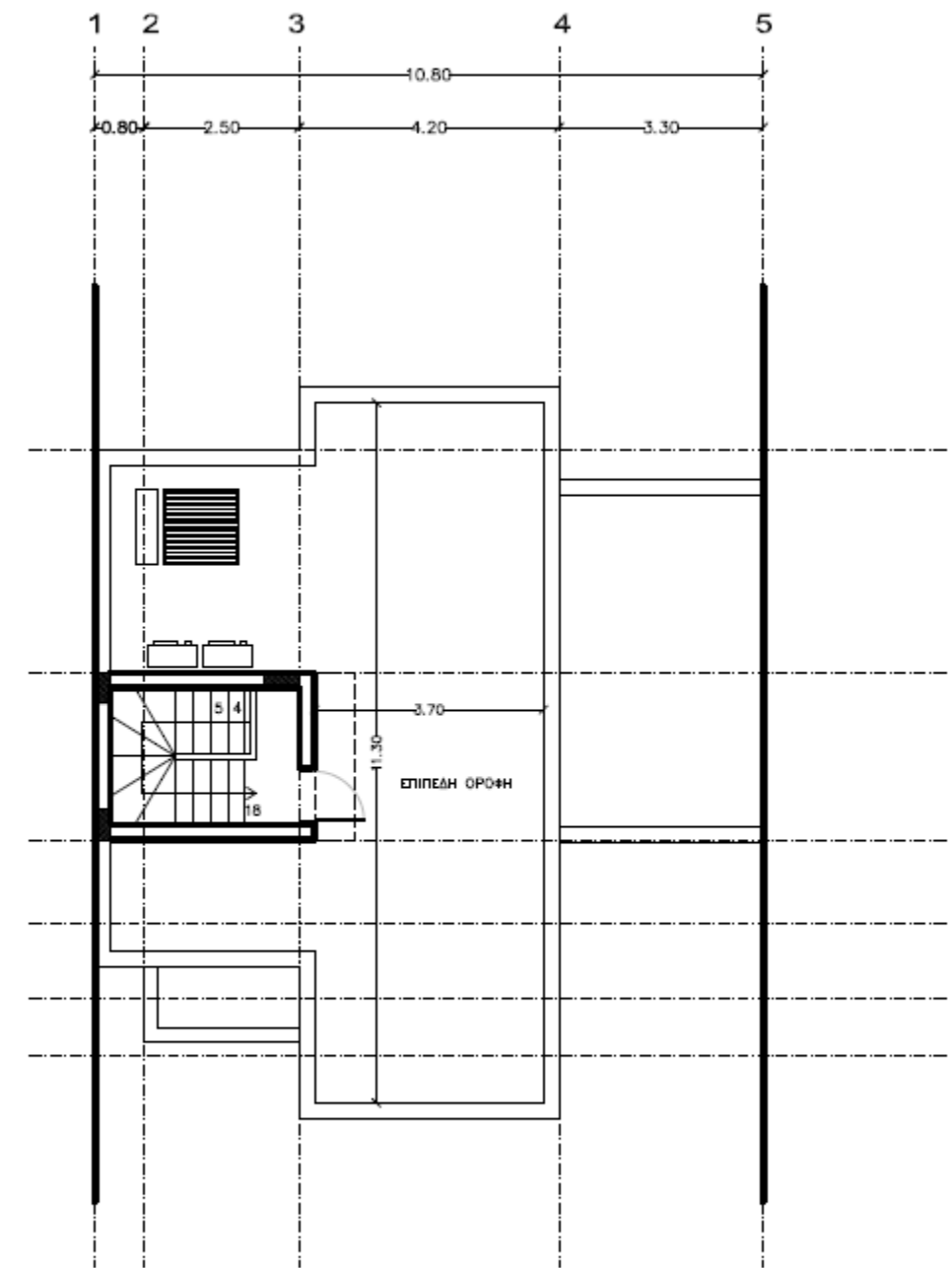
ΚΑΤΟΨΗ ΟΡΟΦΗΣ roof garden
